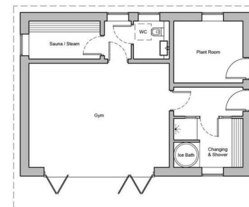
Ground Floor Plan GFA - 68.8m 2 (7,397m 2 )
